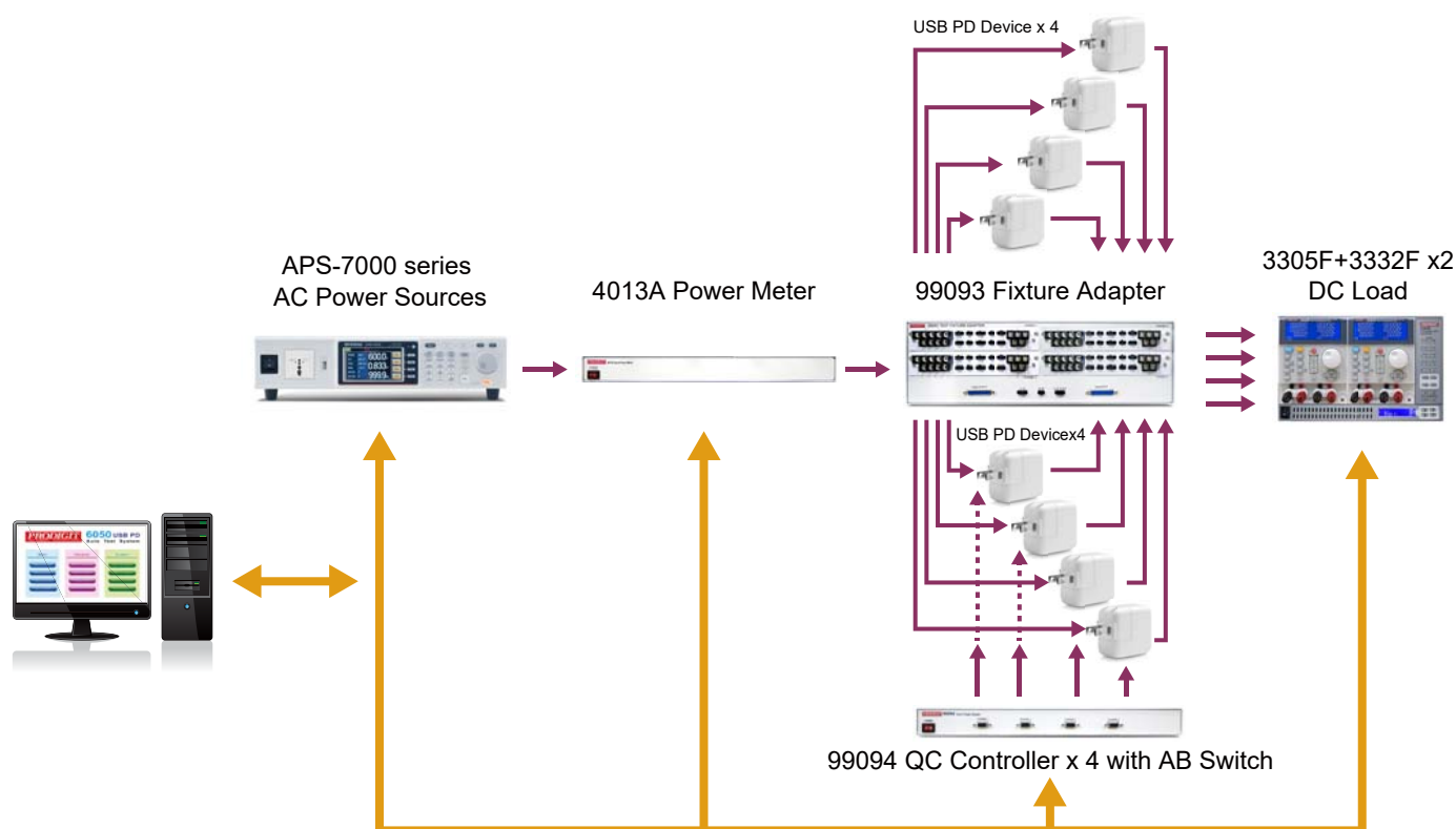
6050-4-A1-X 4 Channel Test System Configuration
