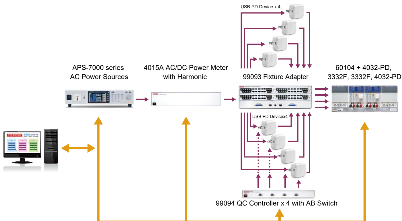
6050-4-C1-X 4 Channel Test System Configuration
